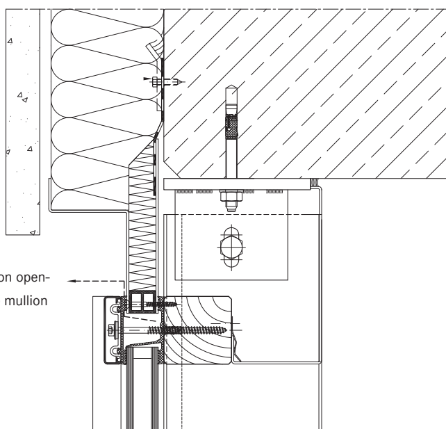
Fig. 2 Ceiling connection
